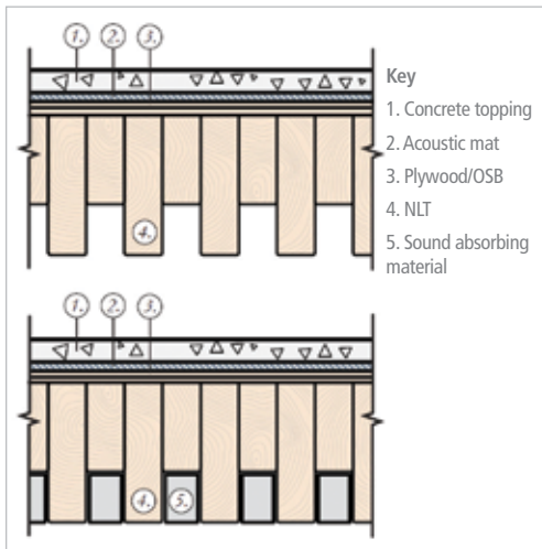
Alternating 2x4 and 2x6 lumber with and without sound absorbing material. Source: NLT US Design and Construction Guide
